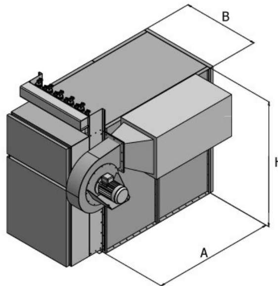
Type 2 Side removal without hopper
