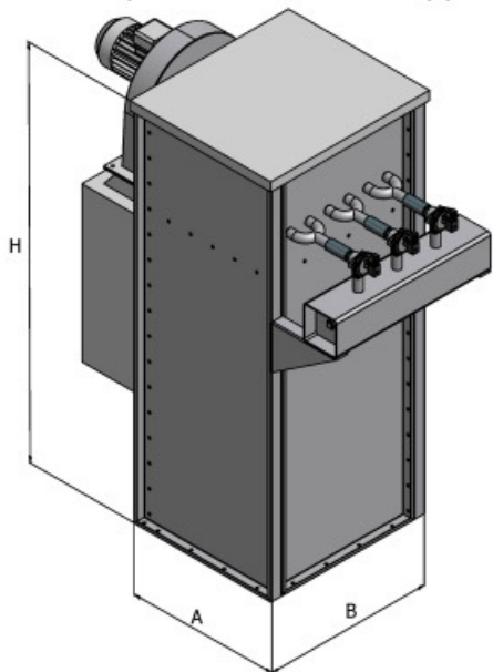
Type 1 Top removal without hopper
